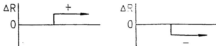
FIG. 6D Change of resistance in magnetoresistive change portion
